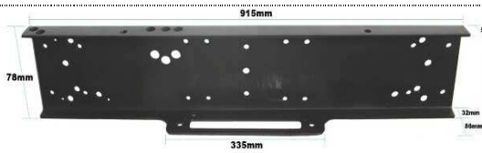
INSTALLATION PLATE
